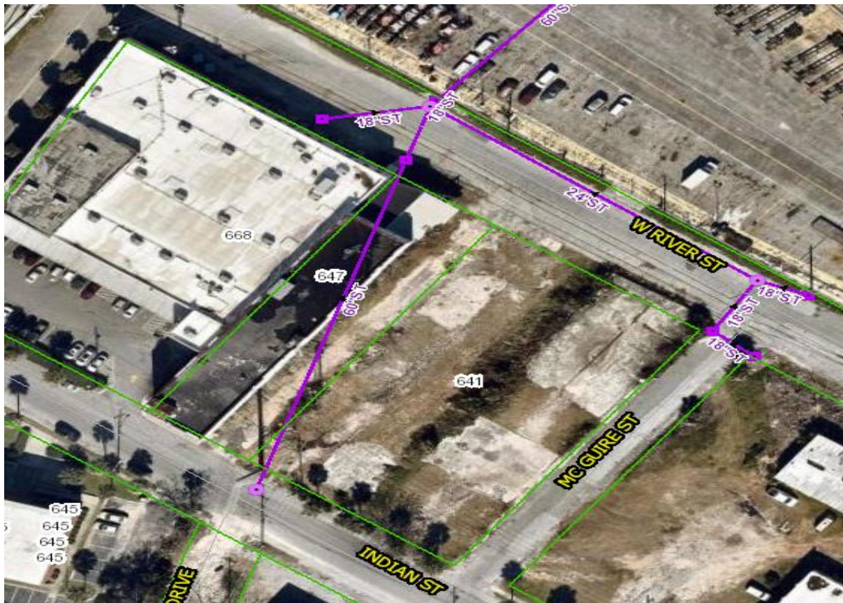
60 inch Stormwater Sewer Line
