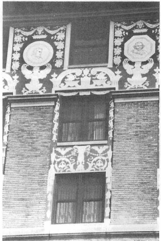
Fig. 11. The Hotel Washington, Washington, D.C. (1916-1917), is notable for its decorative sgraffito surfaces. Stucco panels under the cornice and around the windows feature classical designs created by artists who incised the patterns in the outer layer of red-colored stucco while still soft, thereby exposing a stucco undercoat of a contrasting color. Photo: Kaye Ellen Simonson.
