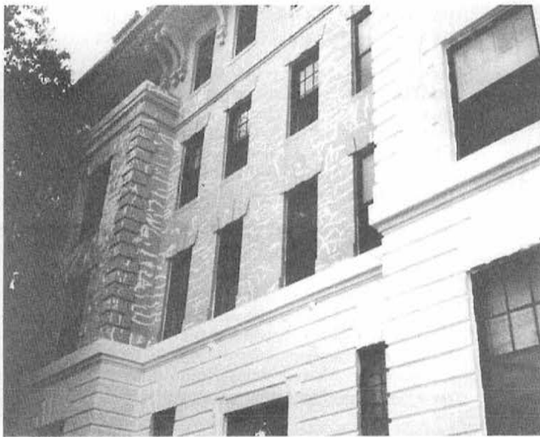
Fig. 13. (a) In preparation for repainting, hairline cracks on this Mediterranean style stucco apartment building were filled with a commercial caulking compound; (b) dirt is attracted and adheres to the texture of the caulked areas, and a year after painting, these inappropriate repairs are highly obvious. Photos: Anne Grimmer.
